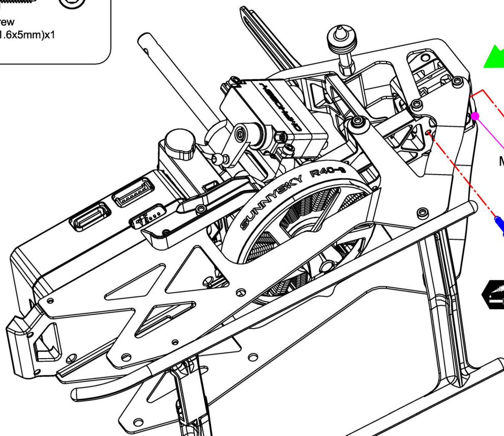
Tail Boom
