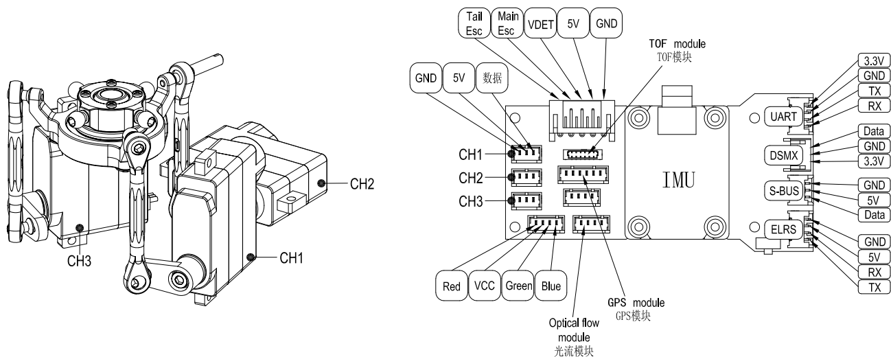
Servo Centering and Pitch Setting 舵机中位和螺距设定
